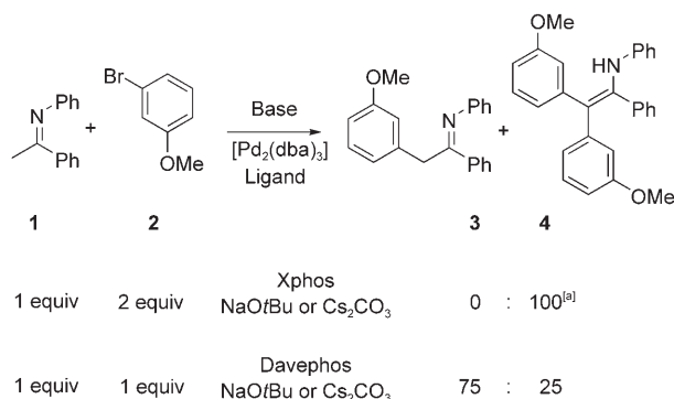
Scheme 2. Pd-catalyzed \alpha -arylation of imine 1 . Reaction conditions: [Pd 2 (dba) 3 ] (4 mol %), 2:1 Pd/ligand molar ratio, 1.4 equiv base, dioxane, 110 °C, 14 h. Xphos = 2-dicyclohexylphosphino-2',4',6'-triisopropylbiphenyl. Davephos = 2-dicyclohexylphosphino-2'-( N,N -dimethylamino)biphenyl. [a] Yield of isolated 4 when Cs 2 CO 3 was employed as base: 76%.
